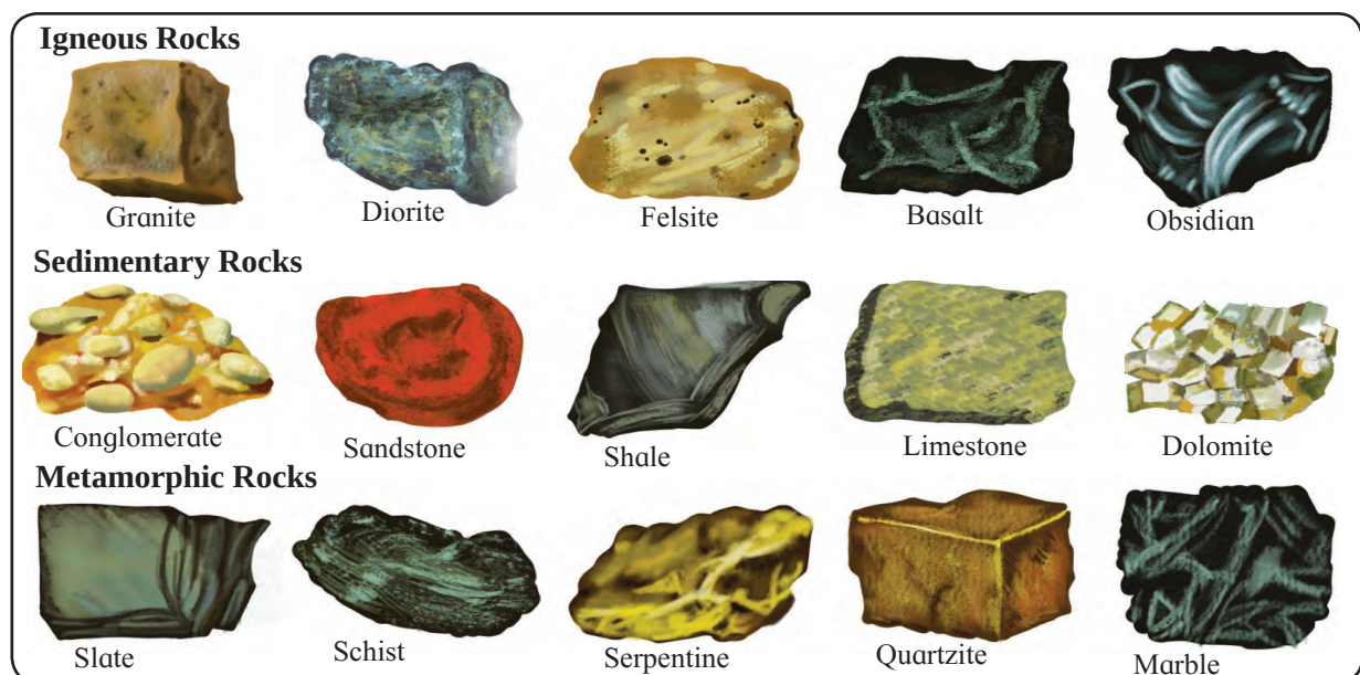
Fig 1.3 : Rock Specimens
