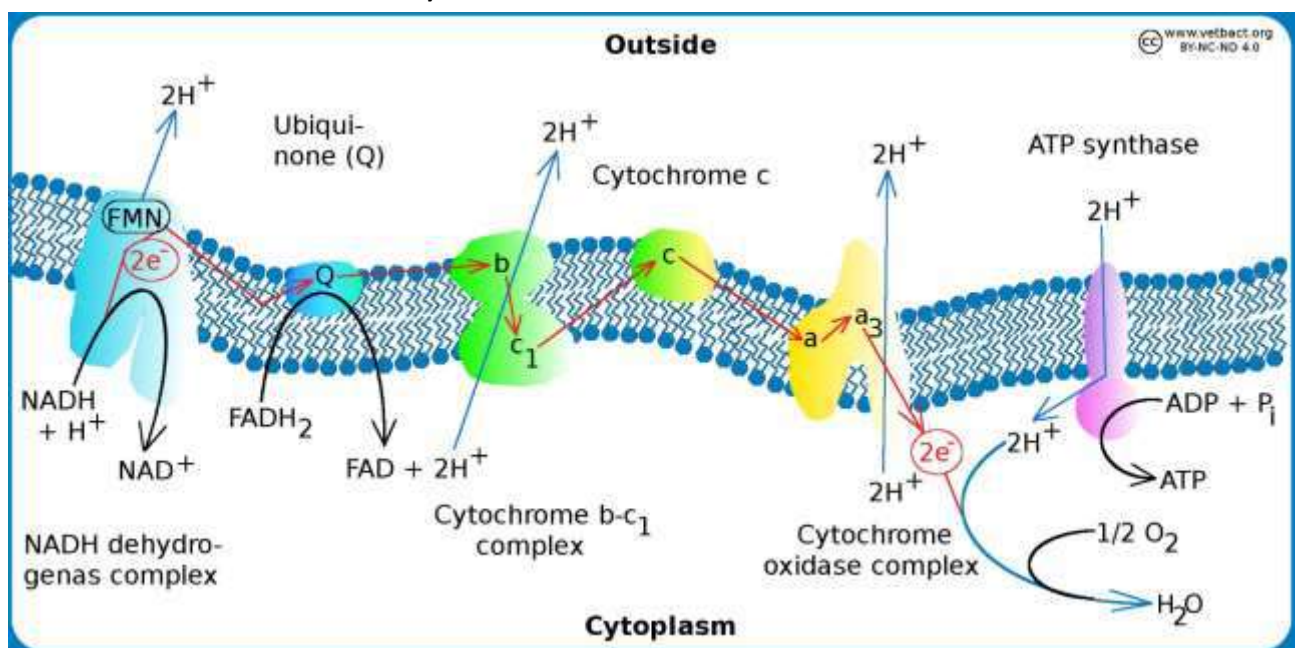
Figure 1. Schematic view of the electron transport chain in bacteria with aerobic metabolism. It shows a sequential oxidation steps where sufficient energy is liberated to permit synthesis of ATP.
