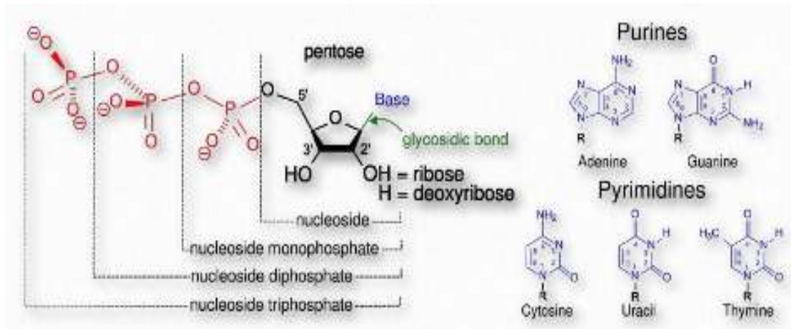
Fig.1 Precursors of DNA
