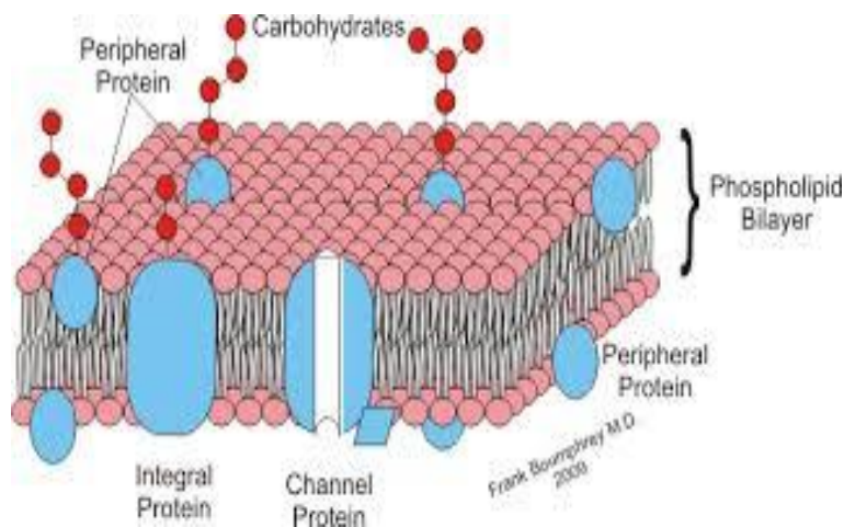
Fig. 6: Cell Membrane
