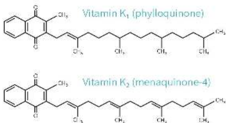
Fig. 17. Structure of Vitamin K
