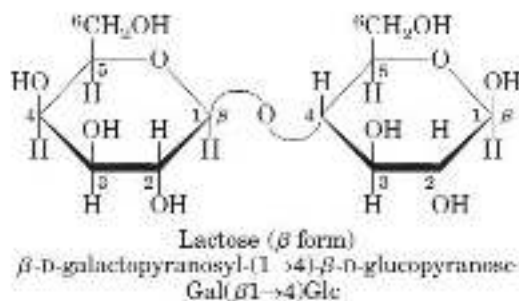
Fig. 14: Structure of lactose
