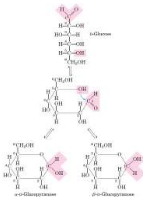
Fig. 11: Cyclic structure of glucose
