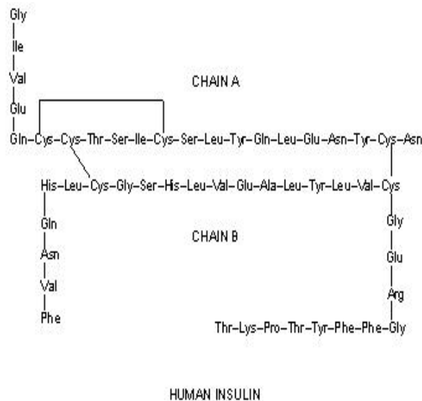
Fig. 5. Structure of insulin
