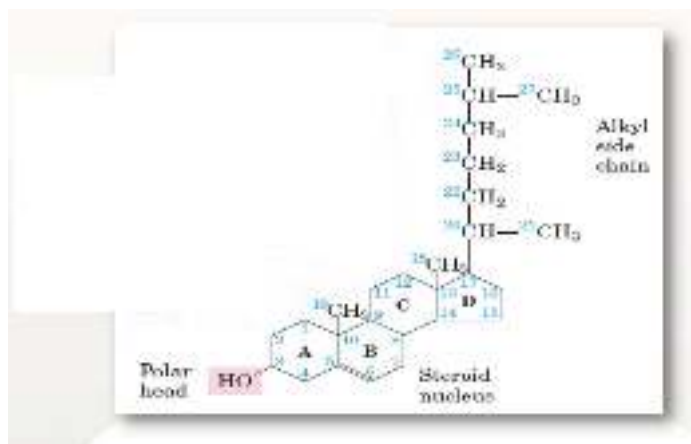
Fig. 5: Structure of cholesterol
