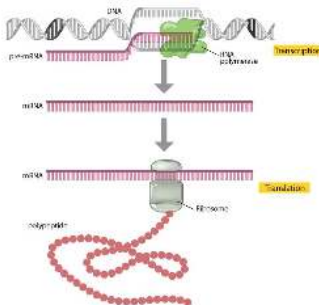
Fig. 5: RNA metabolism
