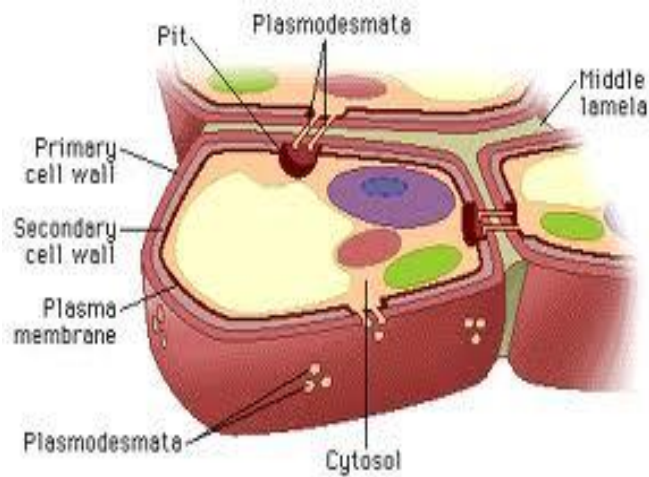
Fig. 2: Cell Wall
