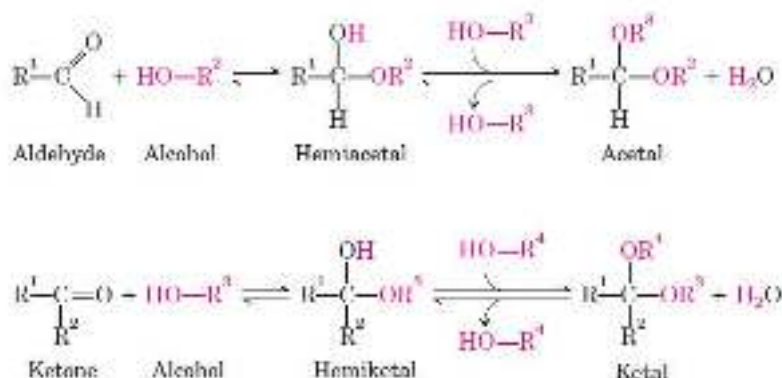
Fig 10: Formation of hemiacetals and hemiketals
