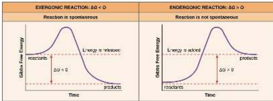
Fig. 16 Exergonic and Endergonic reaction
