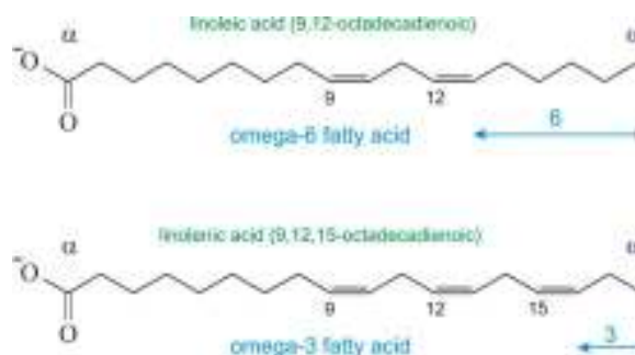
Fig. 6: Omega-3 and 6 fatty acids
