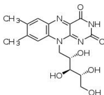
Fig. 7. Structure of Vitamin B2
