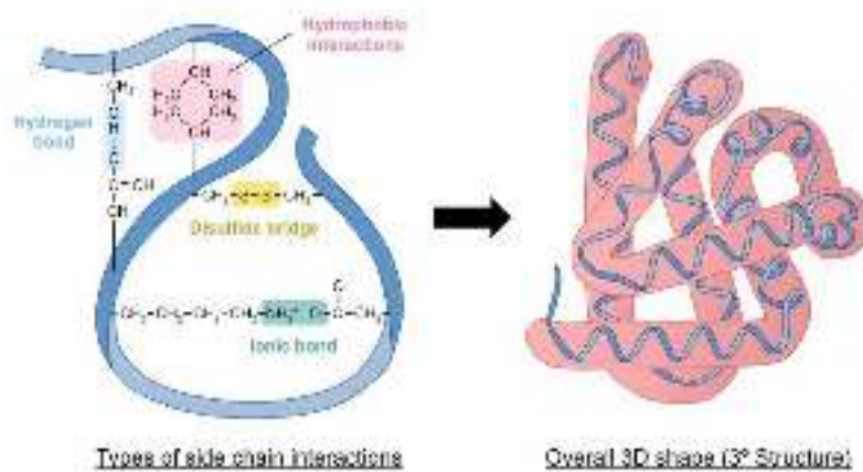
Fig. 8: Tertiary structure of protein
