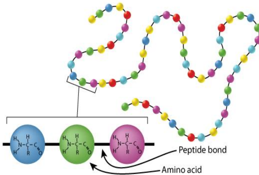
Fig. 2: Primary structure of protein
