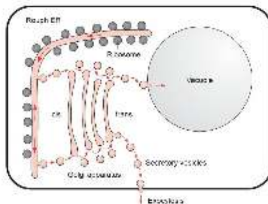
Fig. 10: Scheme of interplay between ER and Golgi apparatus in the transfer of proteins from ER to the vacuoles and in the secretion of proteins from the cell.
