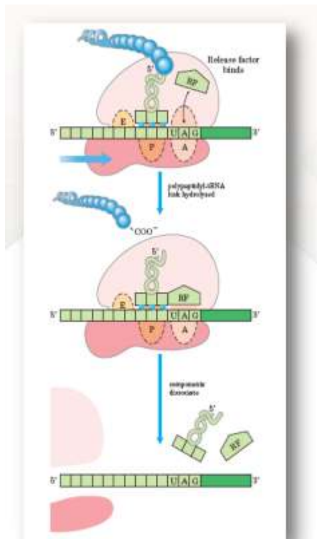
Fig. 15. Termination phase of translation
