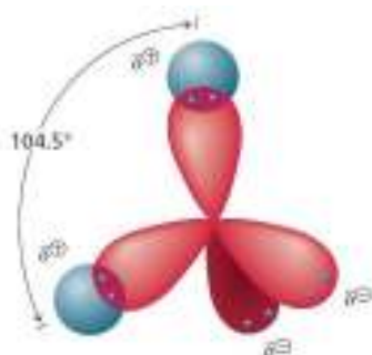
Fig. 12 Structure of water
