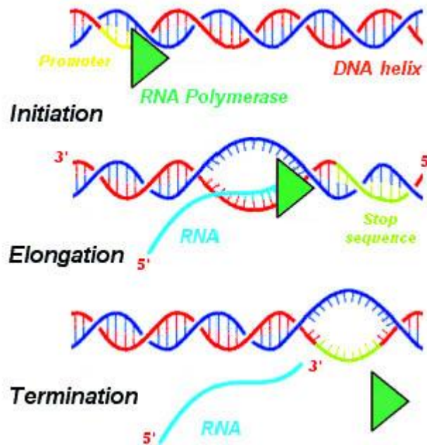
Fig. 7 Process of transcription
