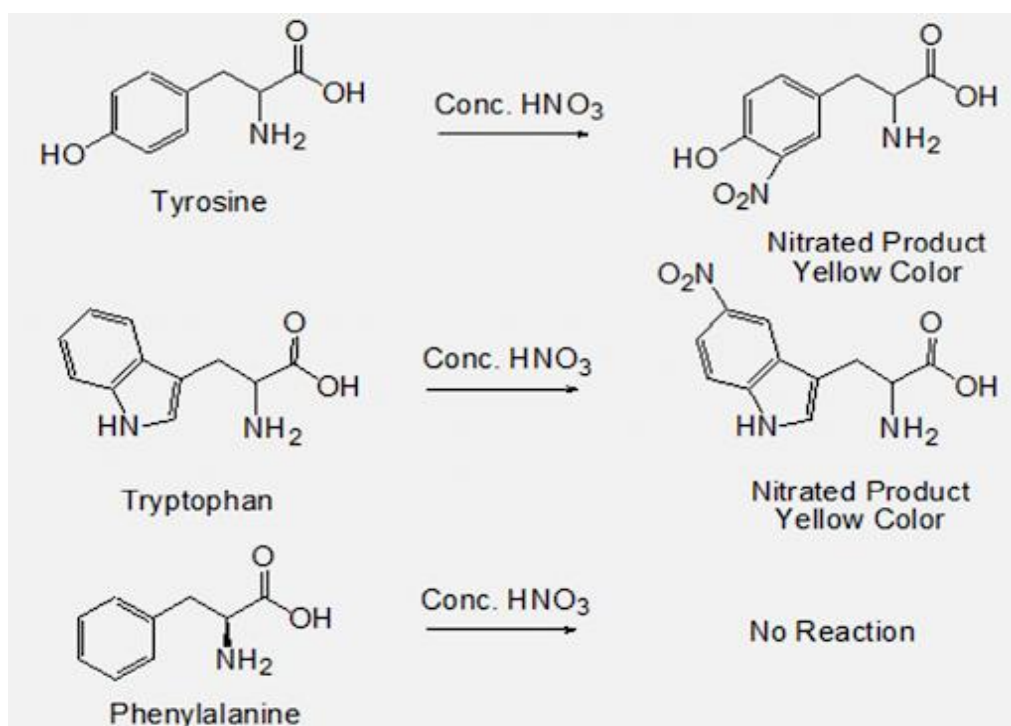
Fig. 11 Xanthoproteic reaction
