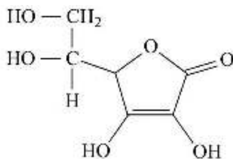
Fig. 18. Structure of Vitamin C
