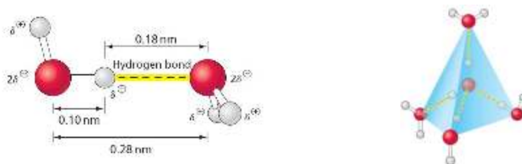
Fig. 14 Hydrogen bond
