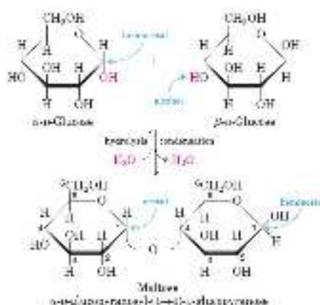
Fig. 13: Structure of maltose
