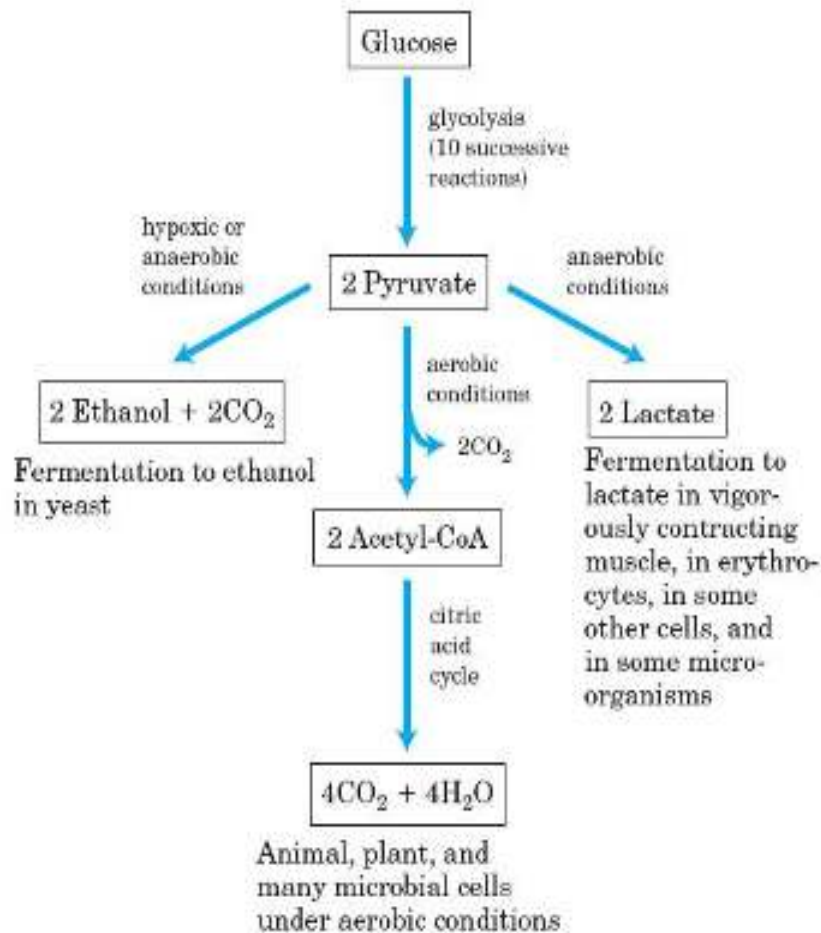
Fig. 3 Three possible catabolic fates of the pyruvate formed in glycolysis.
