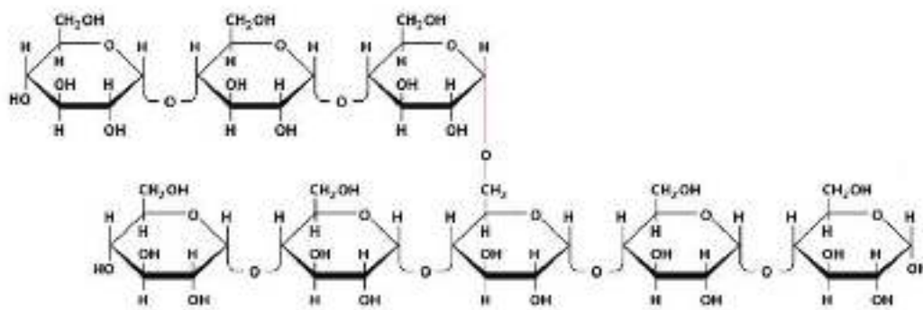
Fig. 17: Structure of glycogen
