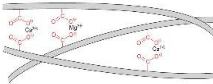
Fig. 5: Structure of Pectin
