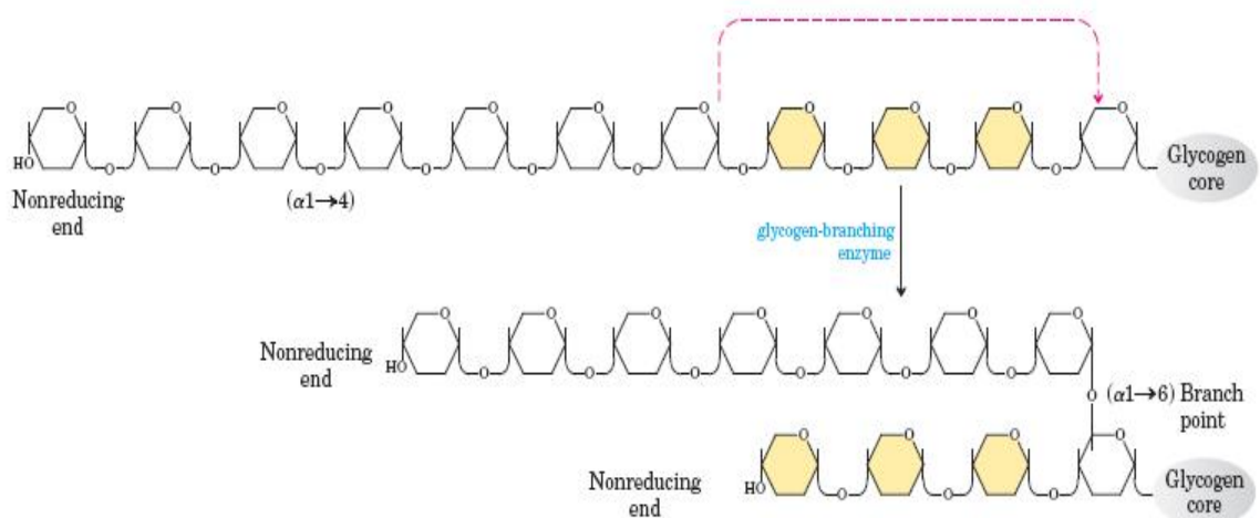
Fig. 8 Branching in glycogen
