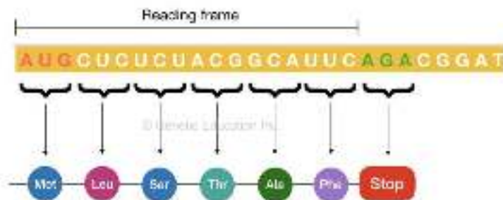
Fig. 11 The example of a ORF with start and stop codon
