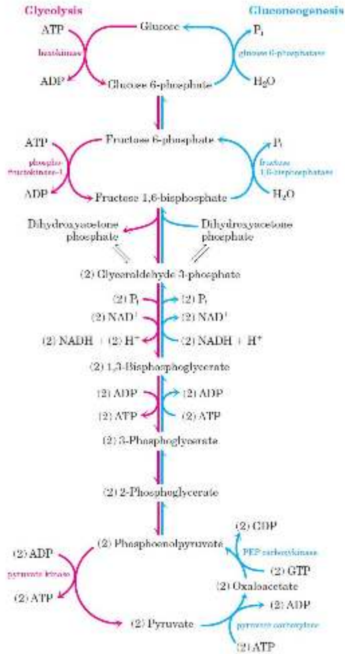
Fig. 4 Glycolysis and gluconeogenesis
