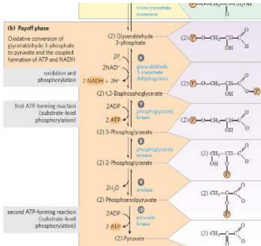
Fig. 2 Pay-off phase of Glycolysis
