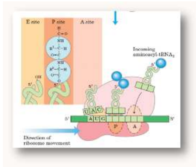
Fig. 14. Elongation phase of translation
