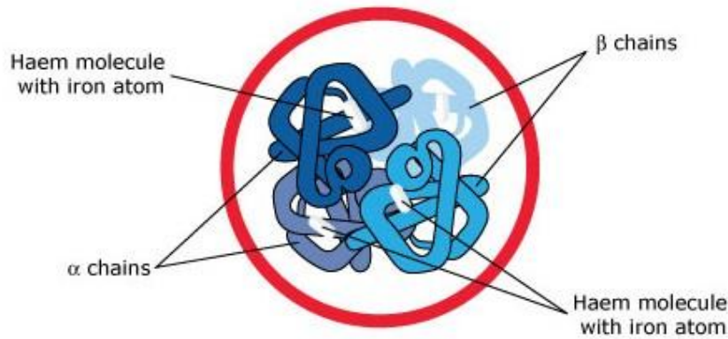
Fig. 9: Haemoglobin molecule
