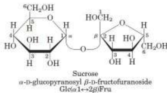
Fig. 15: Structure of sucrose
