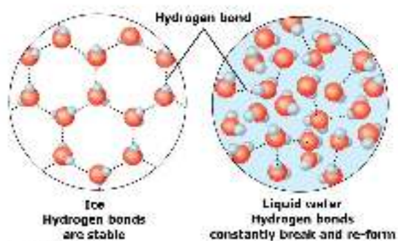
Fig. 15: Hydrogen bond formation in water molecules
