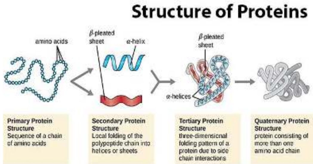
Fig. 1: Different levels of protein structure
