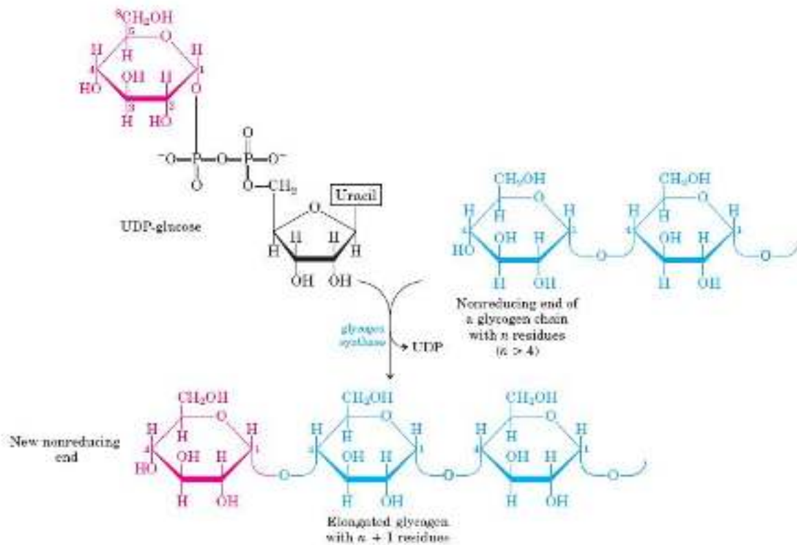
Fig. 7 Glycogenesis
