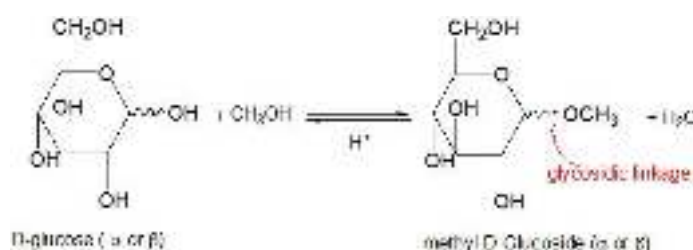
Fig. 21 Formation of glycoside
