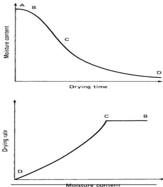
Fig. 3. (a) and (b) Drying curves. The temperature and humidity of the drying air are constant and all the heat supplied to the food surface by convection
