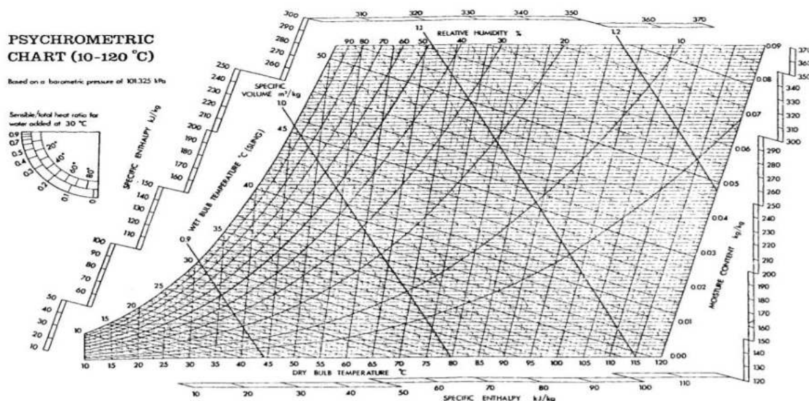
Fig 1. Psychometrics chart
