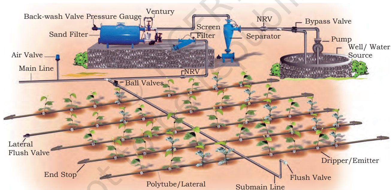
Fig. 1.13: Component and layout of a drip irrigation system
