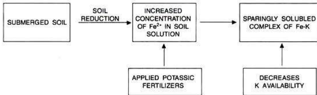
Figure 3 A schematic representations for the transformation of potassium in submerged soil
