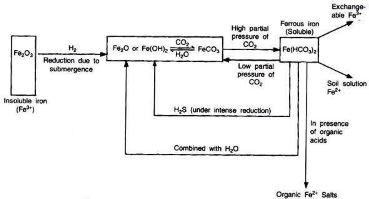
Figure 4 A schematic representations for the transformation of iron in submerged soil
