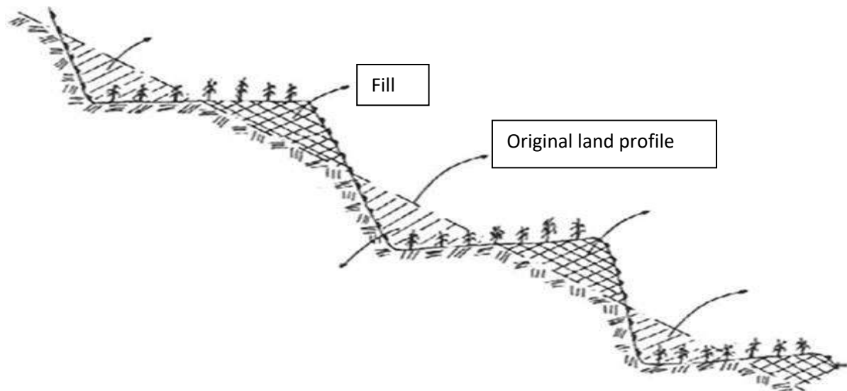
Figure 11 A sketch of a typical bench terrace (FAO 2000)
