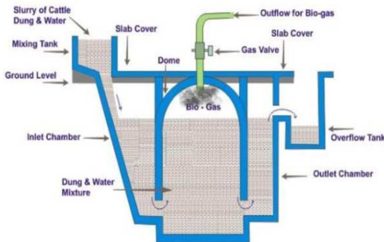
Fig. 2. Fixed dome type bio-gas plant
