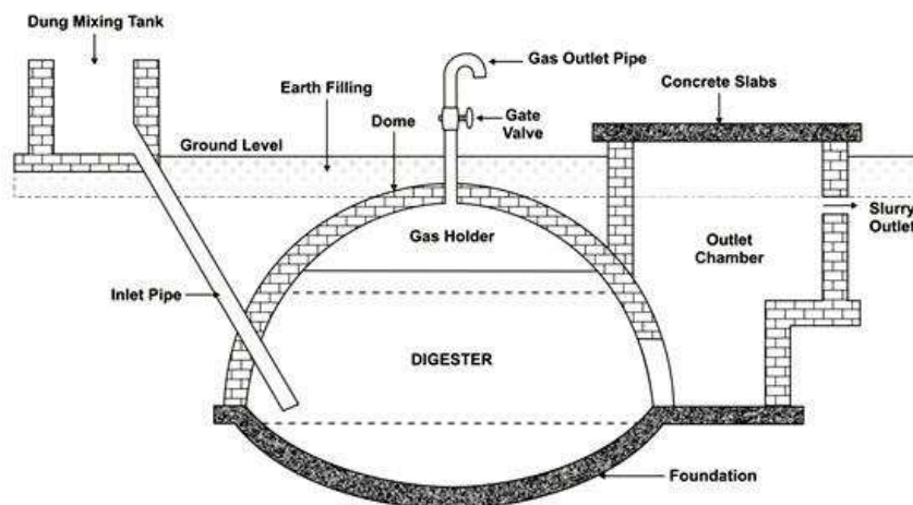
Fig. 3. Schematic diagram of a Deenabandhumodel biogas plant
