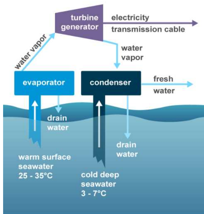
Fig. 6. Ocean thermal energy conversion system
