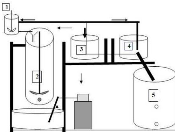
Fig. Biodiesel pilot plant diagrammatic sketch
