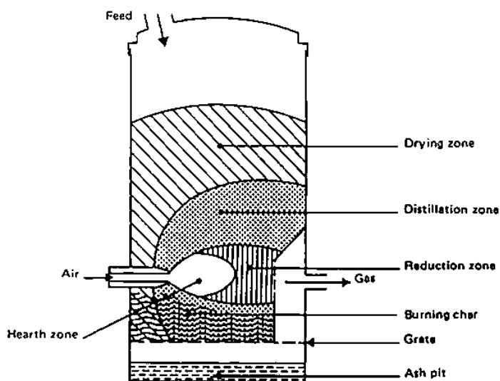
Fig.6. Cross-draft gasifier
