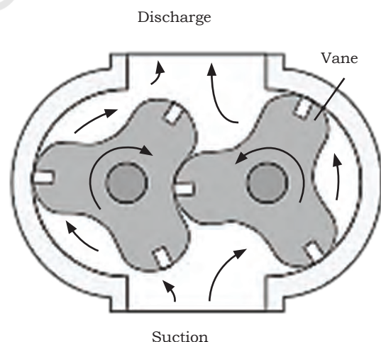
Fig. 2.27: Lobe pump
