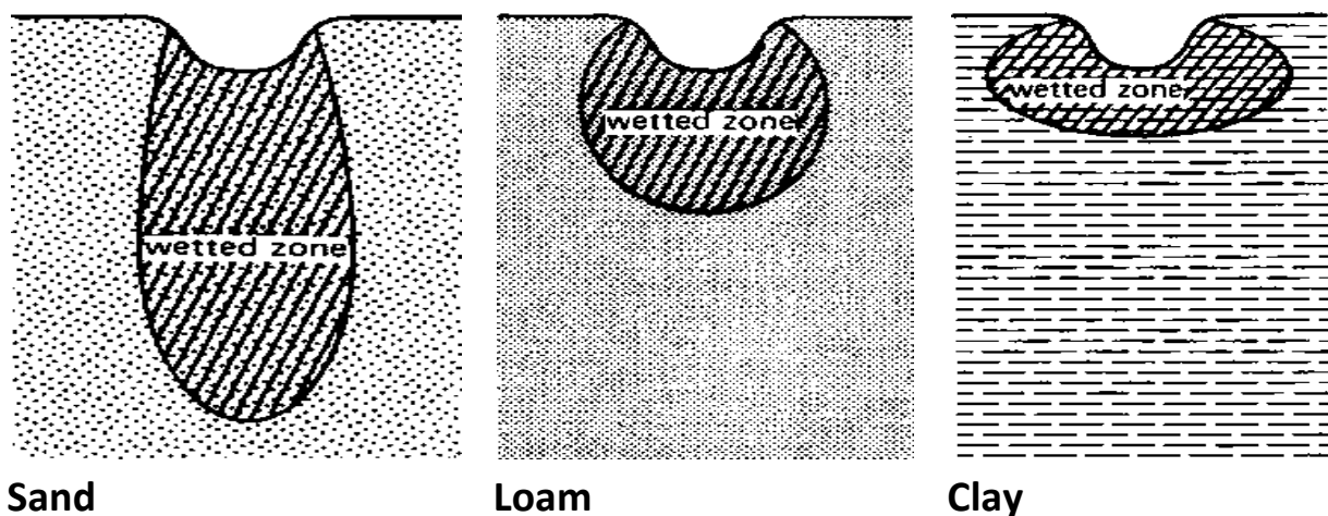
Fig 3. Wetting pattern in furrows in different soil type
