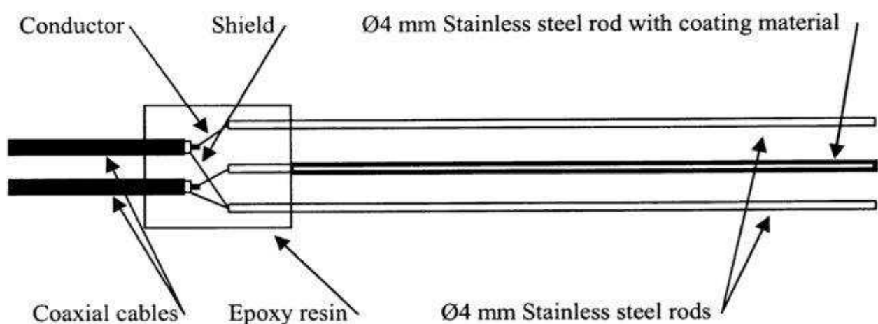
Fig 6 Schematic design of the time-domain reflectometer (TDR) coated-uncoated probe (CUP).
