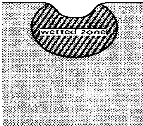
loam
