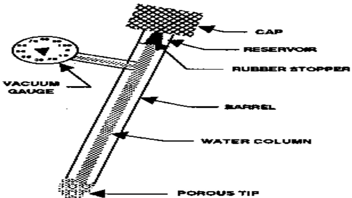
Fig 1 Tensiometer (Source:
