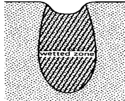
clay
