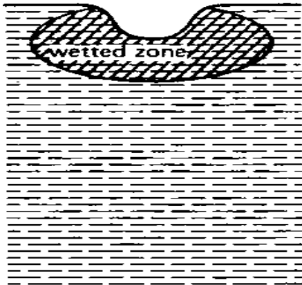
Sand
