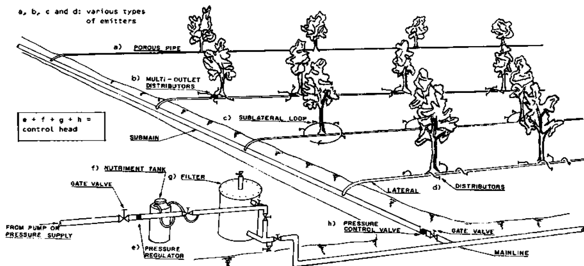
Fig.4 Layout of drip irrigation system
