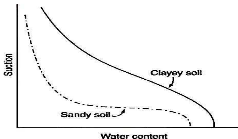
Fig. 1 Effect of soil texture on soil water retention
